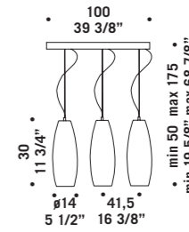
PERONI S14L 3x77W E27 HSGSA/C/UB alogeno chiara clear halogen 3x50W E27 - PAR 20 HAGS/UB 3x24W E27 FBT fluorescente fluorescent 3 x E27 LED LED light bulb
