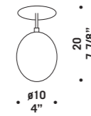
PRO•SECCO F 1x20W-12V G4 HSGST/UB alogeno bispina halogen bi-pin foro incasso \varnothing 7,5 cm trasformatore escluso recess hole \varnothing 7,5 cm transformer not included
